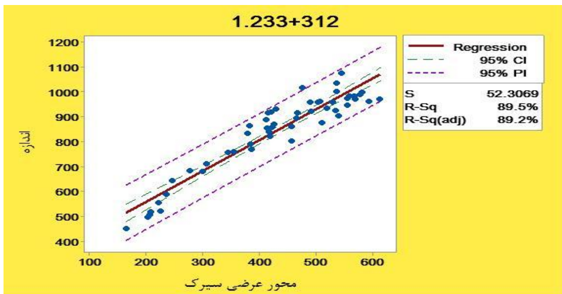
Figure 11: The diagram of the relationship between the size of the N4 and N5 category cirques and their transverse axis in Green heights
