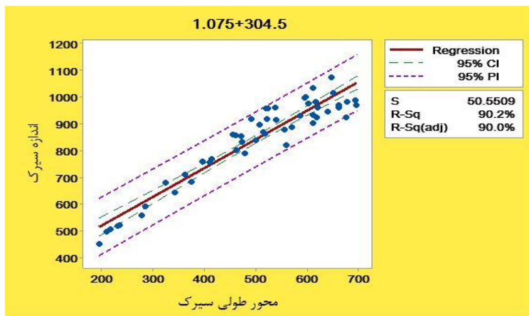
Figure 12: The diagram of the relationship between the size of the N4 and N5 category cirques along their longitudinal axis in Green heights
