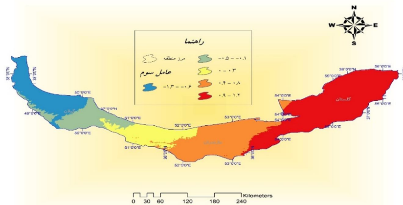
Figure 6: Spatial pattern of the second factor in the region (humidity and precipitation factor)
