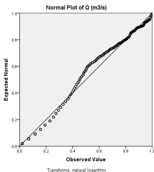
Figure 9: Normality Test Plot
