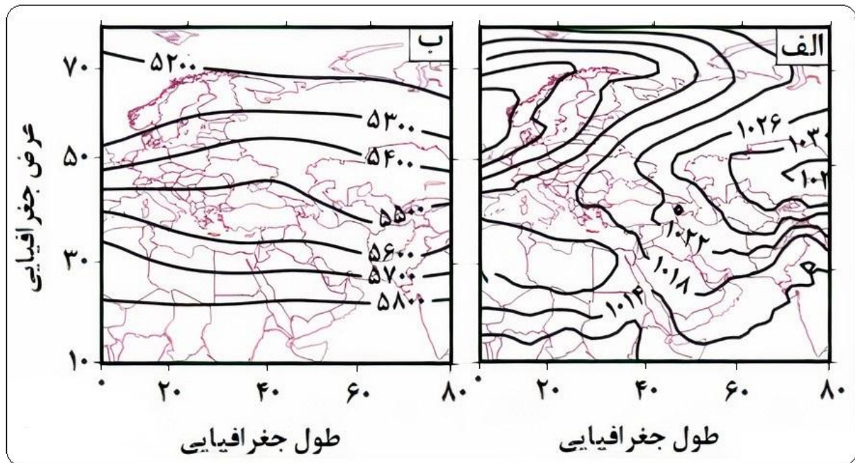
Figure 10: a) Average Sea level pressure (hctopascal), b) Average level height of 500 hectopascals (geopotential meters) for the fifth pattern
