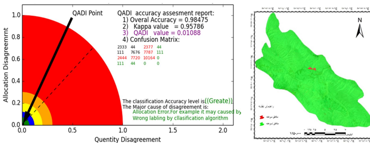
Figure 10: Classification map and result of accuracy assessment with change percentage of the combination of NIR & NBRI57
