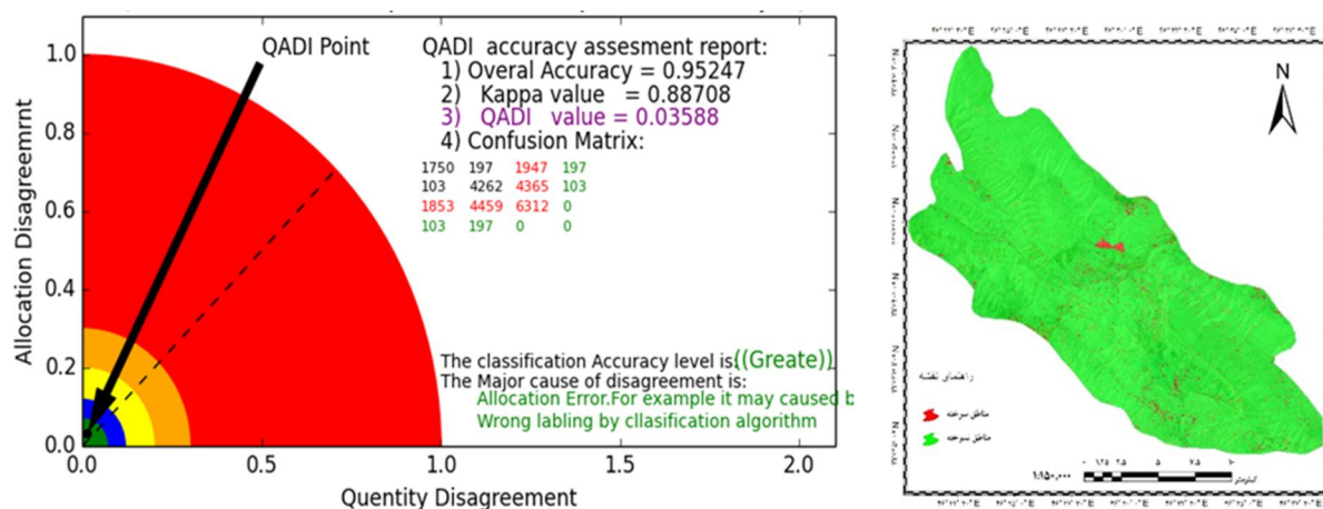
Figure 9: Classification map and result of accuracy assessment with change percentage of the NMDI
