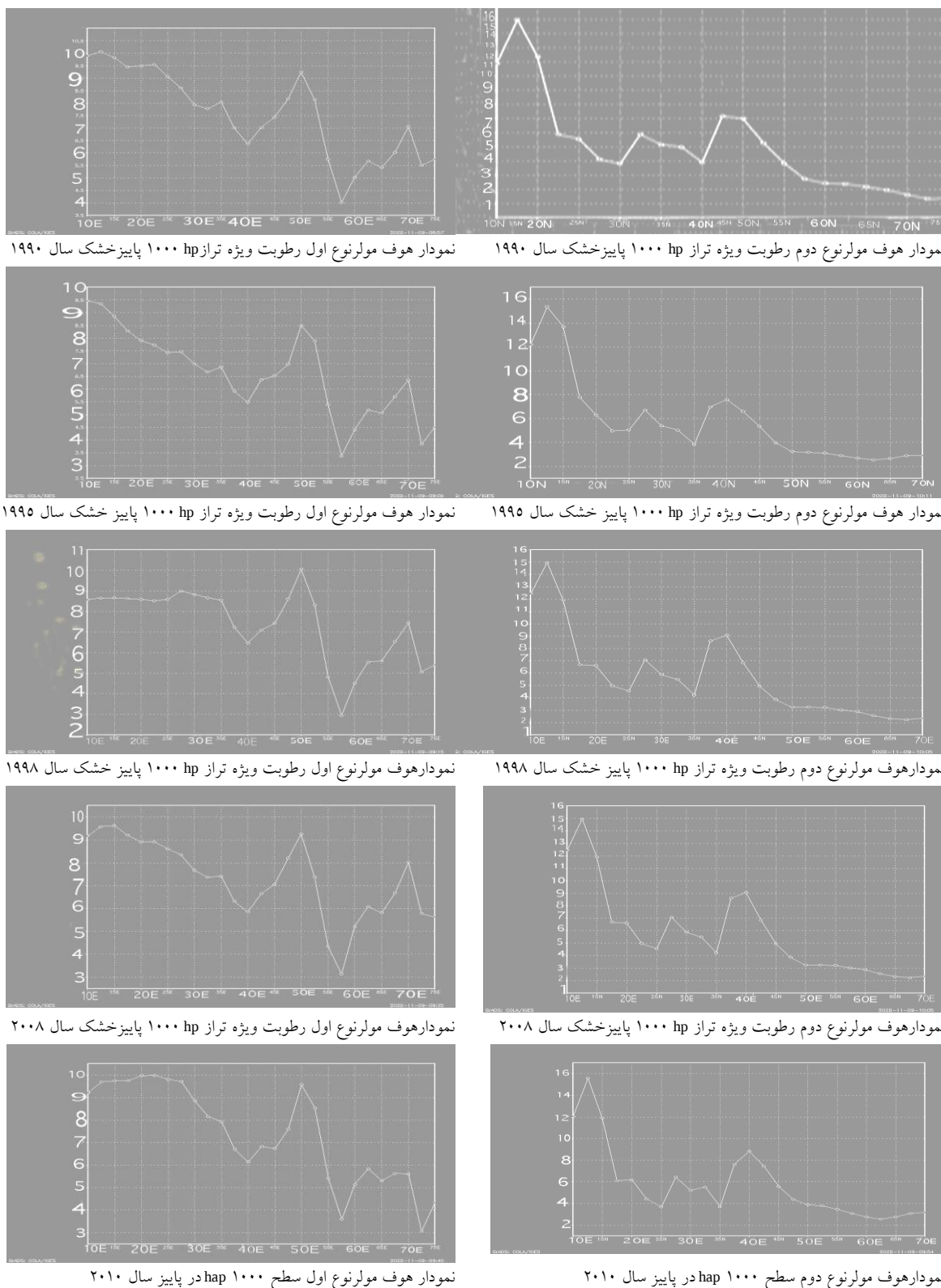
Figure 29: The first and second type of Hof-Mueller diagram in level of 1000 hpa in autumn seasons 2010, 2008, 1998, 1995, 1990
