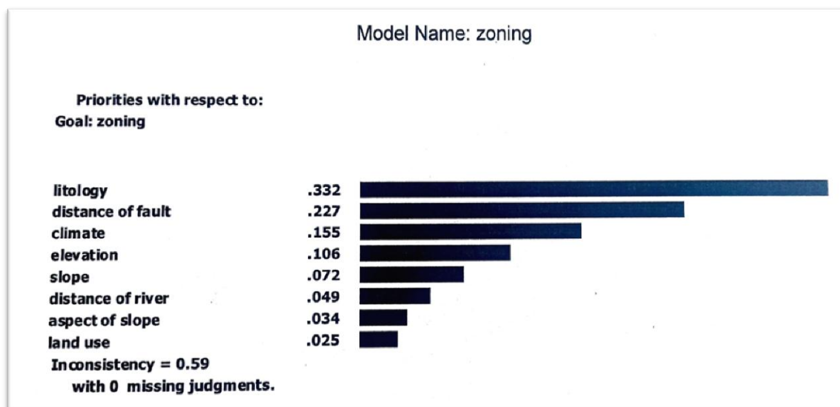
Figure 13: Coefficients obtained from pairwise comparison of the main criteria effective in the development of karst hierarchical analysis process
