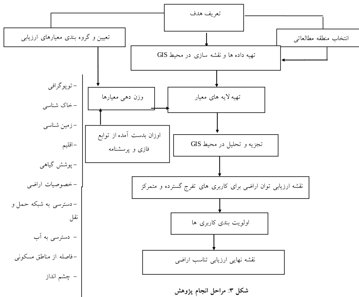
Figure 3: Research flowchart
